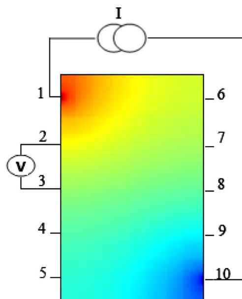
Figure 6 Strategy of diagonal electrodes.
