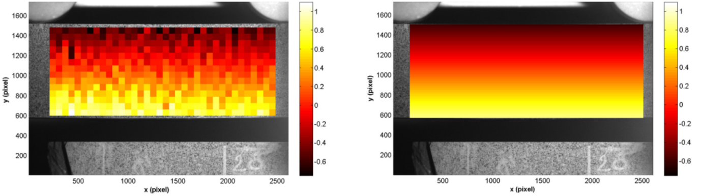
Fig. 5. Horizontal strain field after 45 h of creep. On the left, DIC with Q4 elements of 64 \times 64 pixels; on the right, DIC with the global beam shape functions.
