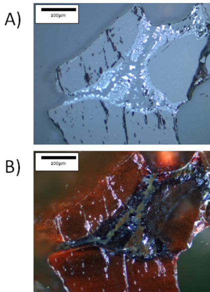
Fig. 19. Micrograph of calcined olivine at 1400°C–48 h. (A) Bright field, (B) Dark field.
