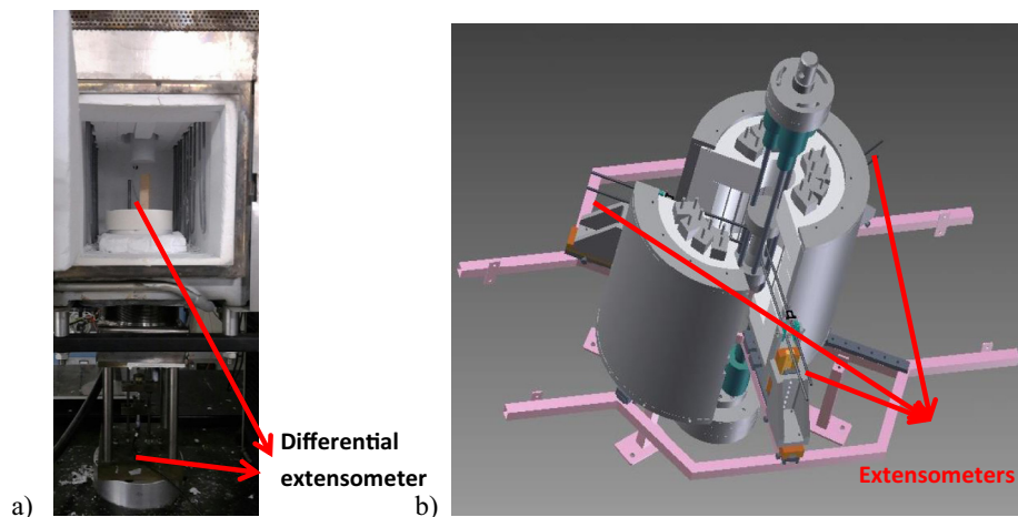
Fig. 13. (a) Compression test using a differential extensometer, (b) Tensile test.
