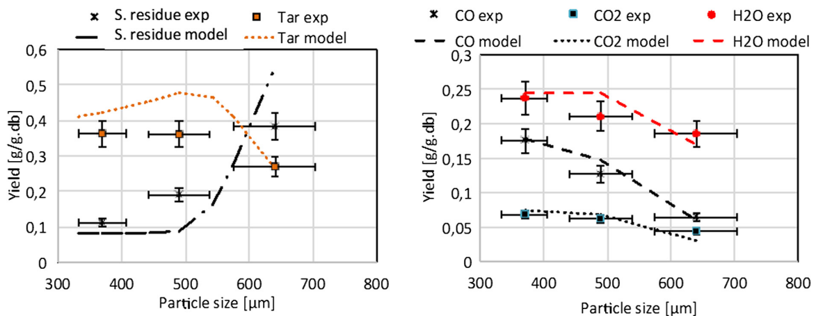
Fig. 5. Comparison between the experimental yields and modeled ones for the different particle sizes (T = 550 °C).
