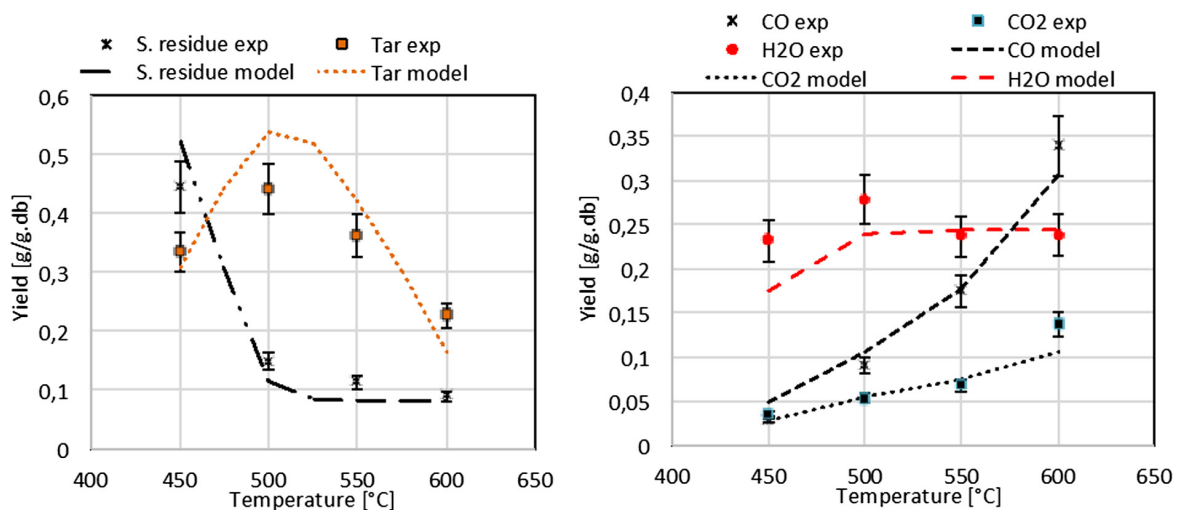
Fig. 4. Comparison between the experimental yields and modeled ones for the different reaction temperatures (PS = 370 μm).
