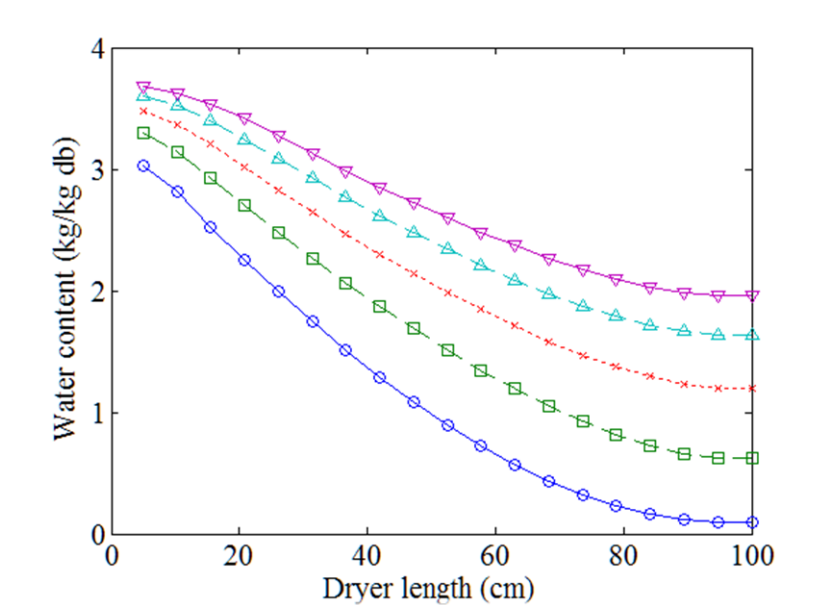
Figure 12: Simulated water content profiles with varying stirring speeds
