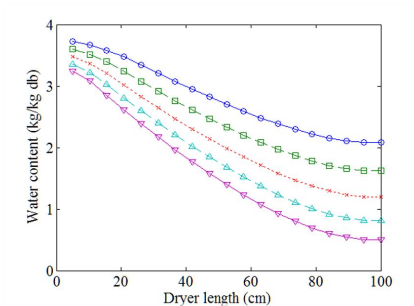
Figure 11: Simulated water content profiles with varying SS inlet flow rates
