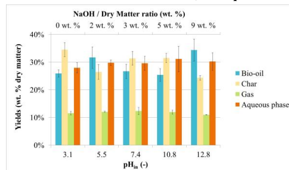
Figure 7: Yields of products obtained by HTL of blackcurrant pomace at various initial pH of the feed and NaOH loadings (operating temperature = 300 °C; holding time = 60 min)
