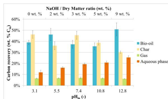
Figure 8: Carbon distribution in products obtained by HTL of blackcurrant pomace at various initial pH of the feed and NaOH loadings (operating temperature = 300 °C; holding time = 60 min)
