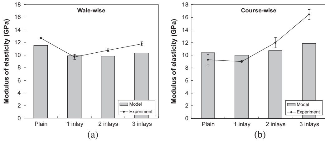
Fig. 7. Experimental and computed elasticity modulus of basalt knit reinforced composites in the wale (a) and course-wise (b) directions.
