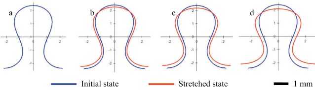
Fig. 4. Tensile behaviour in the course-wise direction of a basalt plain-knit. Comparison of the load/strain curve to experimental data and shape of the loop for several levels of deformation. (For interpretation of the references to colour in this figure legend, the reader is referred to the web version of this article.)
