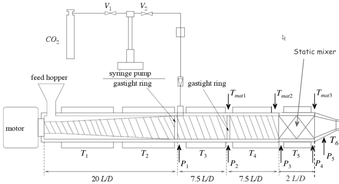
Figure 1. Schematic picture of the foaming system
