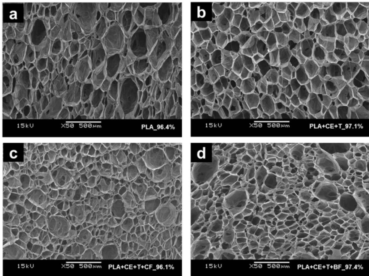
Figure 4. SEM micrographs of the cell morphologies obtained for highly expanded ( \epsilon > 95\% ) PLA foams. The actual porosity values are represented after the abbreviation of the materials within every micrograph.
