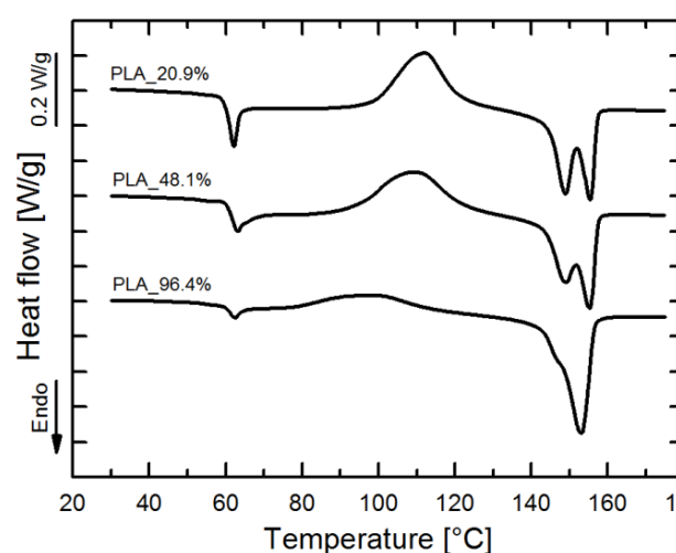
Figure 5. DSC curves of PLA foams of increasing porosity. The actual porosity values are represented after the abbreviation of the materials within the graph
