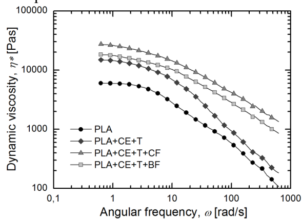
Figure 2. Dynamic viscosity as a function of angular frequency for neat and additive containing PLA
