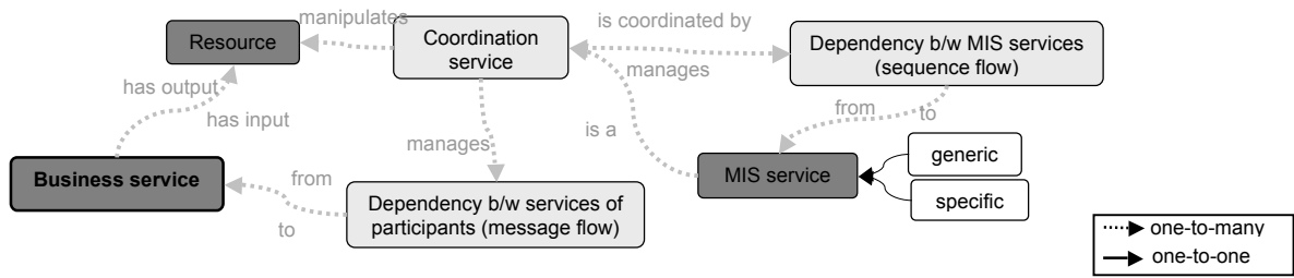
Figure 6 Collaboration Process Ontology (CPO) schema
