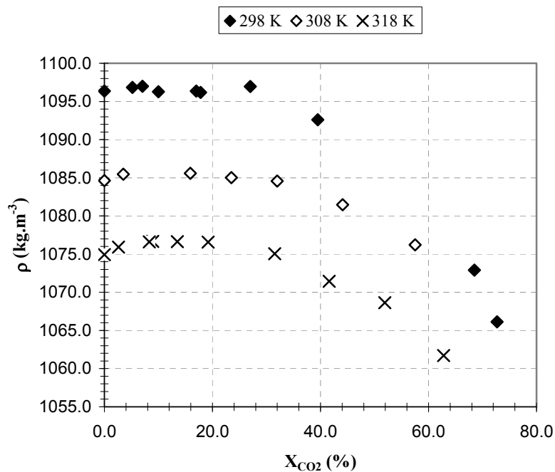
Figure 13. Evolution of liquid density of DMSO-CO 2 with the CO 2 solubility
