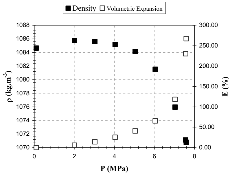
Figure 12. Evolution of liquid density of DMSO-CO 2 and its volumetric expansion at 308 K
